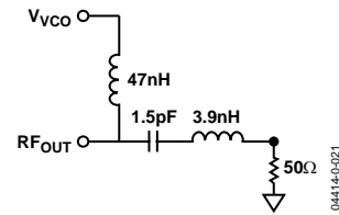
Figure 19. Differential ADF4360-0 Output Stage
