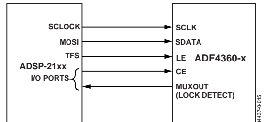
Figure 18. ADSP-21xx to ADF4360-x Interface
