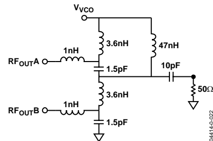
Figure 20. Balun for Combining ADF4360-0 RF Outputs
