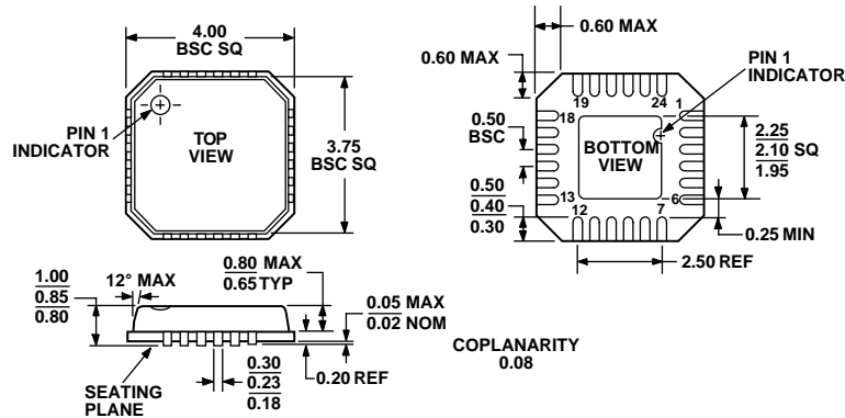
Figure 21. 24-Lead Lead Frame Chip Scale Package [LFCS] (CP-24) Dimensions shown in millimeters
